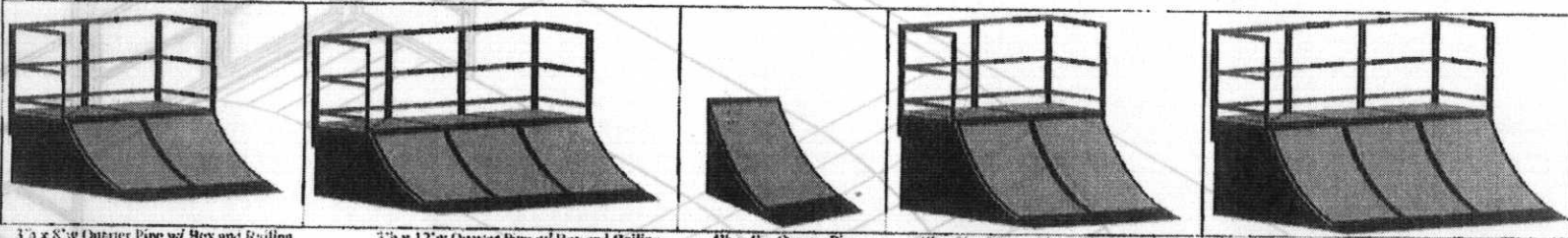
3'h x 8'w Quarter Pipe w/ Box and Railing
