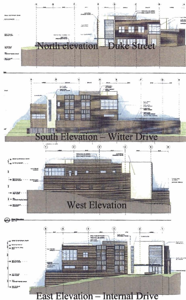
Figure 7. Building Elevations
