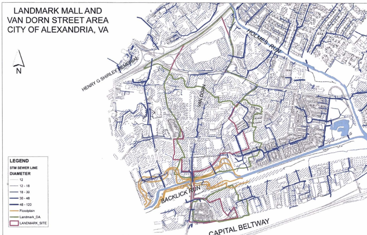
Figure 8-4. Sewer lines in the Landmark/Van Dorn area.
