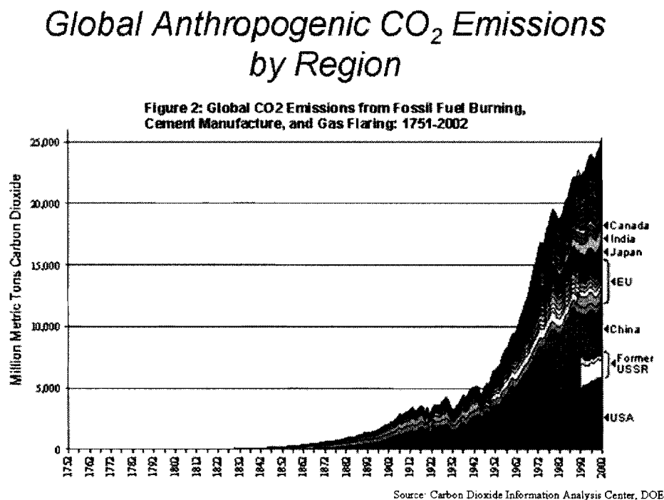
Figure 1. Global Anthropogenic CO 2 Emissions by Region
