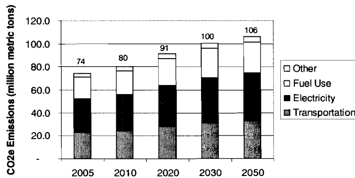
CO 2 e Emissions Projections for the Washington, DC-MD-VA Region
