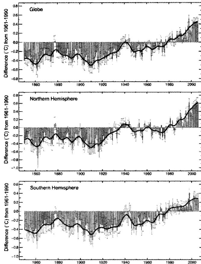
Figure 3. Observed Global Warming
