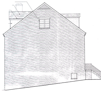
Figure 2 Side elevation
