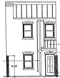
Figure 1 Proposed rear elevation
