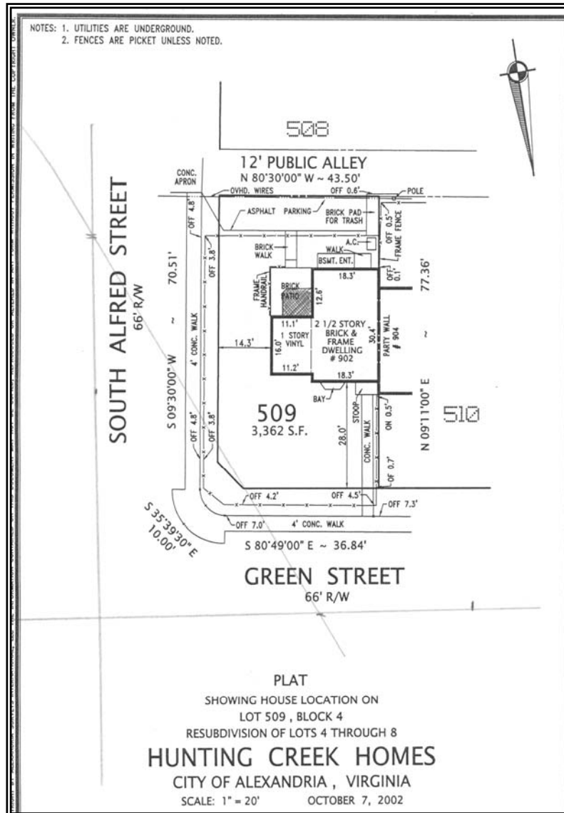
Figure 1: Site plan
