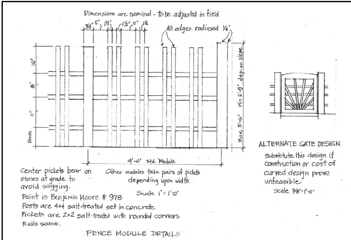
Figure 7. Fence details.
