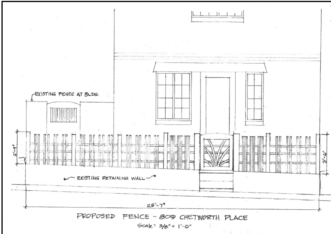
Figure 5. Fence elevation.
