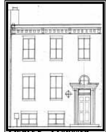
front (north) elevation
